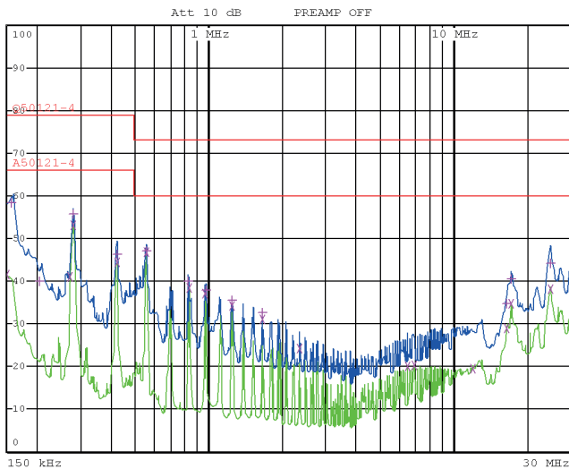
Fig. 8a XRCM60-24: Typ. disturbance voltage at the input ( V_i = 16.8\text{ V} , I_{i, \text{nom}} , resistive load, quasi peak and average)
