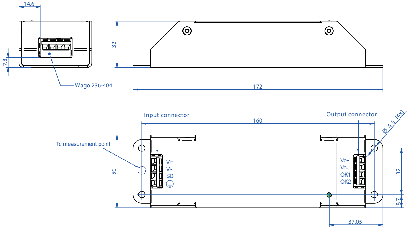
Fig. 10 Case of RCM60 with standard cage clamp terminals, Aluminum, EP-powder coated Weight approx. 350 g
