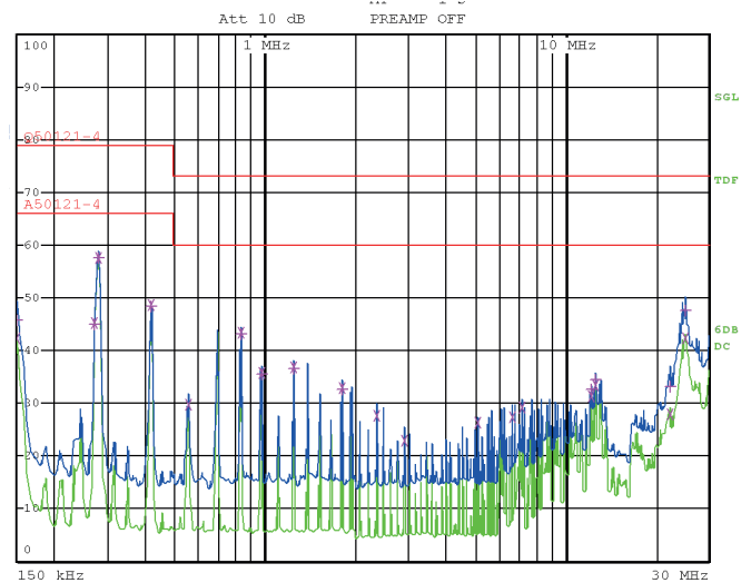
Fig. 8b XRCM60-24: Typ. disturbance voltage at the input ( V_i = 137.5\text{ V} , I_{i, \text{nom}} , resistive load, quasi peak and average)
