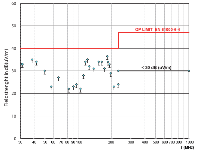
Fig. 9b XRCM60-24: Typ. radiated disturbances in 10 m distance ( V_i = 137.5\text{ V} , I_{i, \text{nom}} , resistive load, quasi peak).
