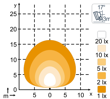
N3102 2400lm Diffused
