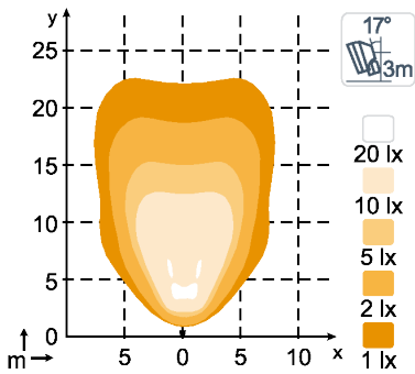
N3102 3000lm Wide Flood
