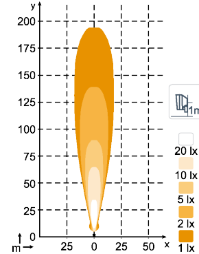
N3102 3000lm High Beam
