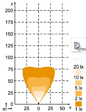
N3102 3000lm Low Beam
