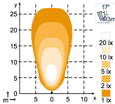
N3102 3000lm Flood
